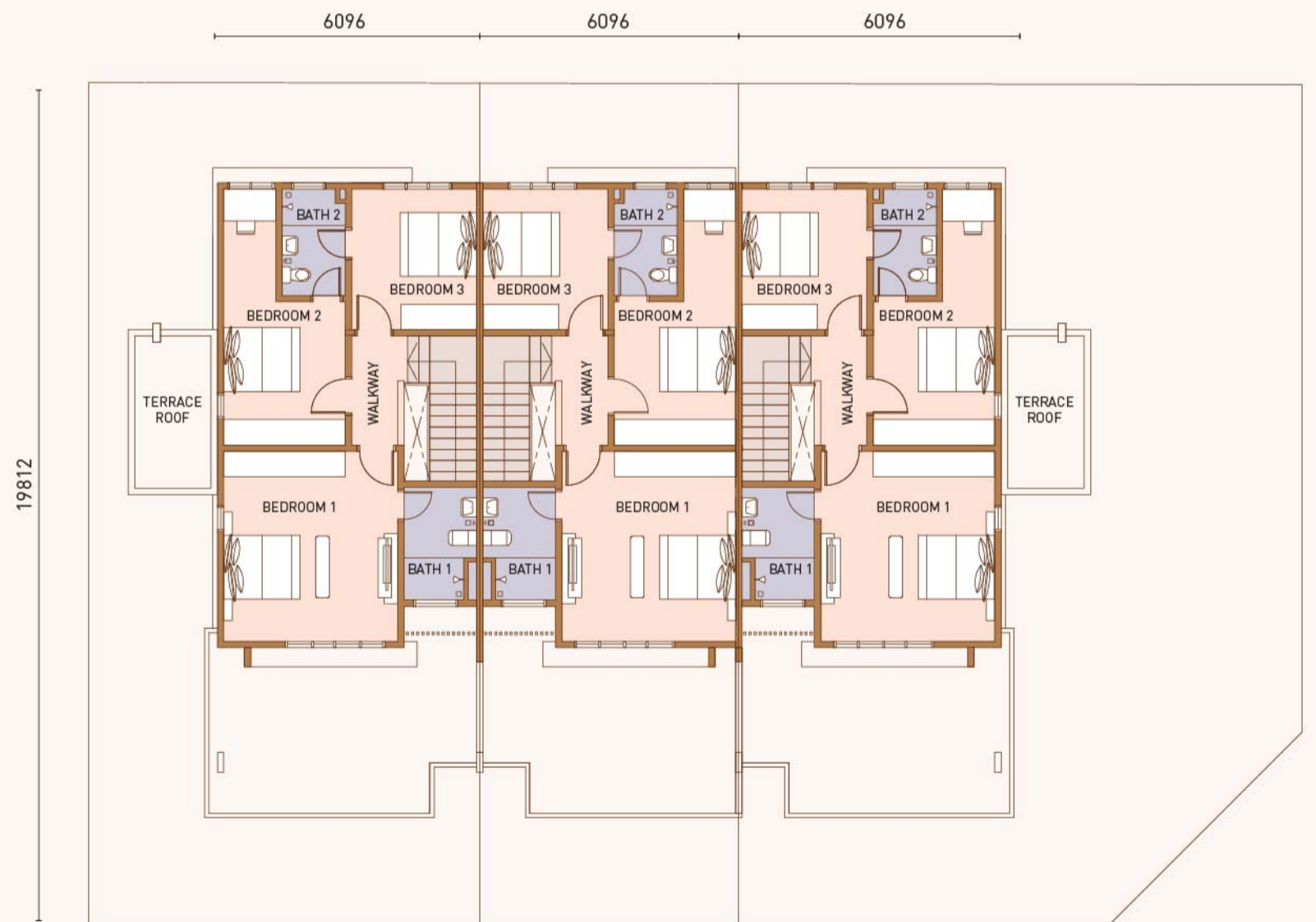
FIRST FLOOR
