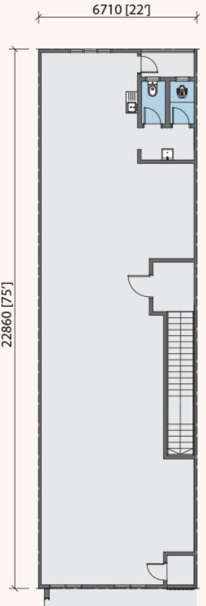
FIRST FLOOR
